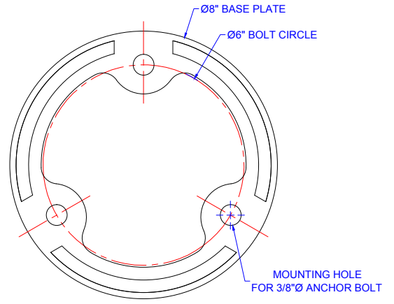
MOUNTING DETAIL
