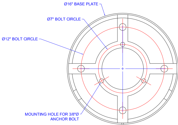
MOUNTING DETAIL
