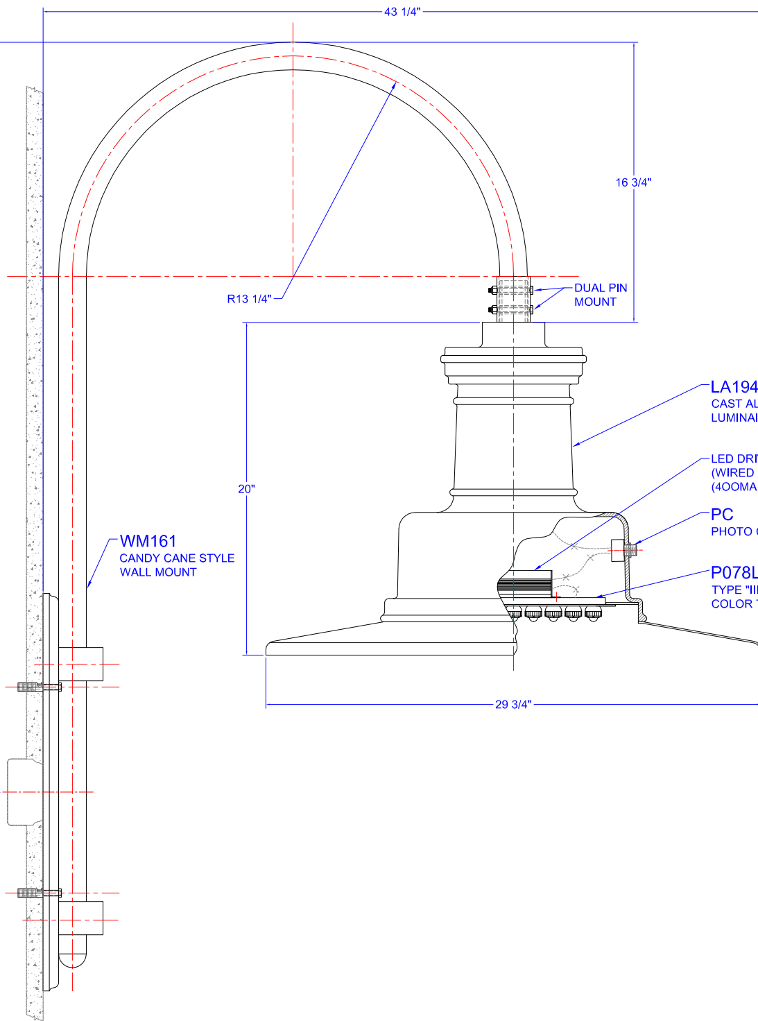
MOUNTING DETAIL
