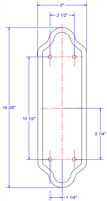
MOUNTING DETAIL
