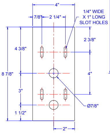
MOUNTING DETAIL
